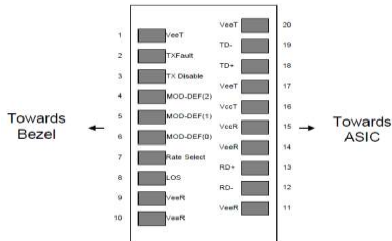
Figure 2: Pin-out of Connector Block on Host Board
