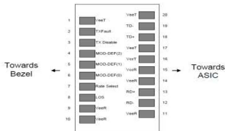
Figure 2: Pin-out of Connector Block on Host Board
