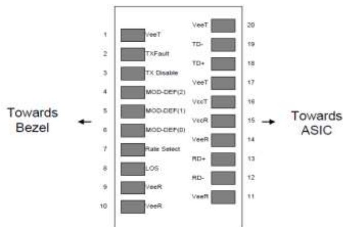
Figure 2: Pin-out of Connector Block on Host Board
