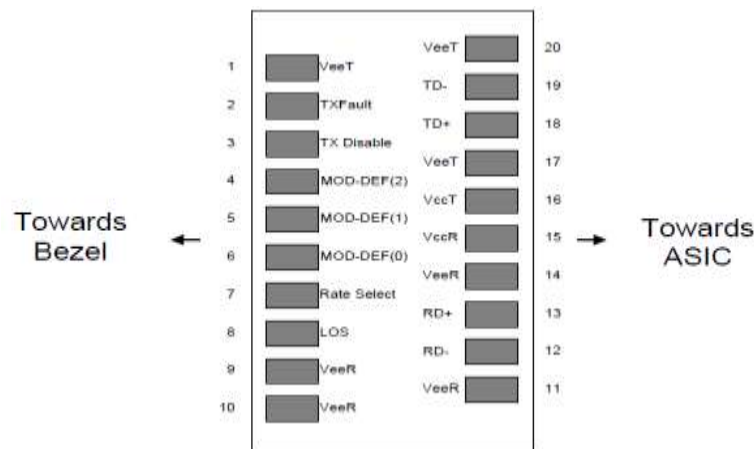
Figure 2: Pin-out of Connector Block on Host Board
