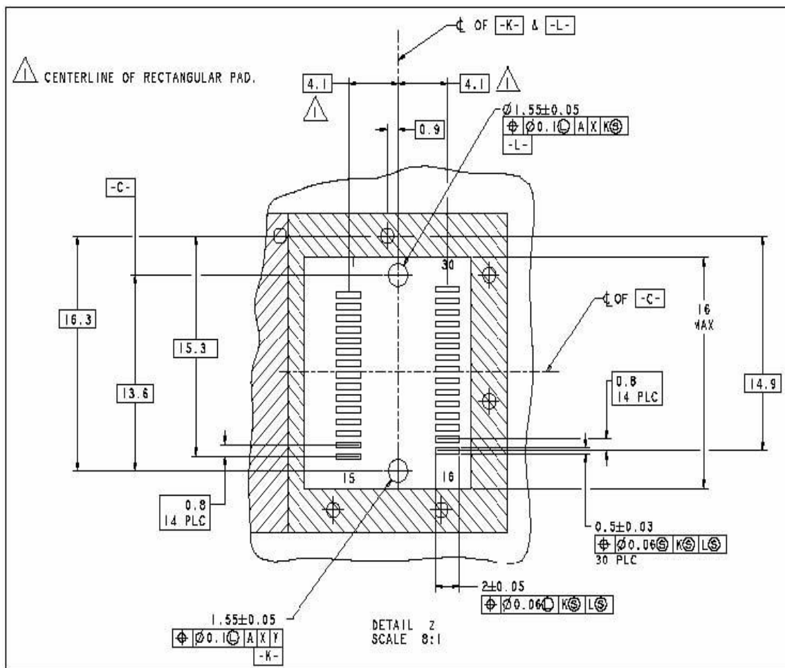
XFP Host Board Mechanical Layout (dimensions are in mm)
