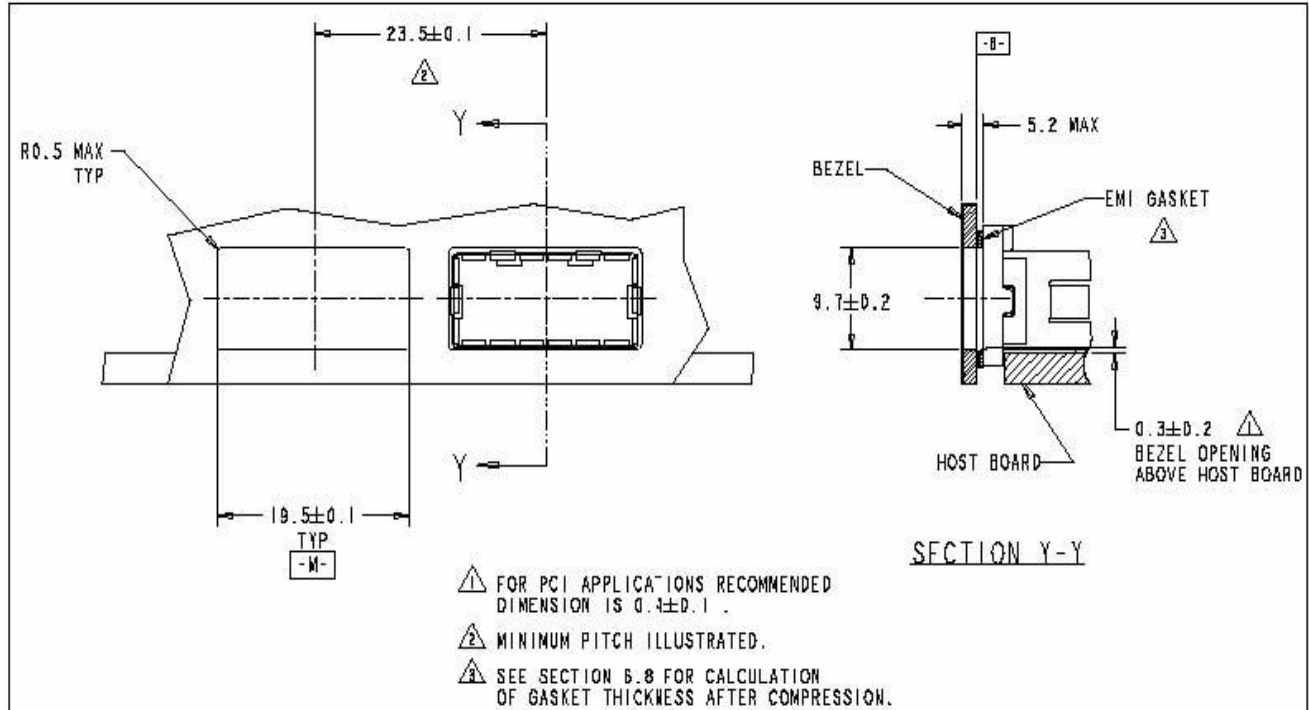
XFDP Detail Host Board Mechanical Layout (dimensions are in mm)
